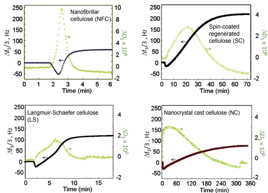
FIGURE 2. Changes in frequency (f) and dissipation (D) for the four model cellulose films subjected to cellulase. Data is shown for the third overtone. Filled squares correspond to frequency and open diamonds correspond to dissipation. The nature of the cellulose films explains the differences in the dissipation curves.
