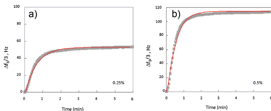
FIGURE 3. The change in frequency shows the hydrolytic activity for the NFC model film. Experimental values are plotted using filled squares and the best fit is indicated with a solid line. The phase modeled is that occurring after the initial cellulase adsorption step. Two different enzyme concentrations were used: a) 0.25% v/v and b) 0.5% v/v. Figures used with permission from the authors.
